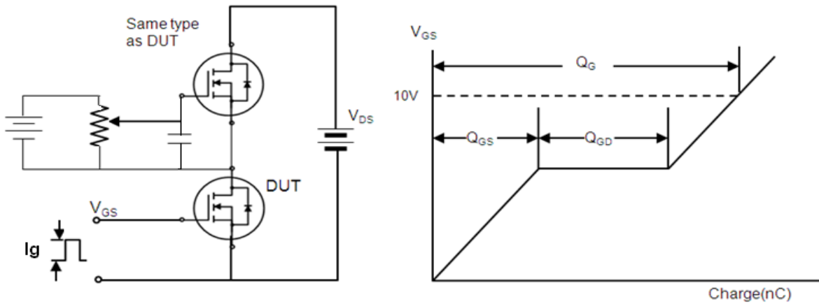
Fig. 15. Gate charge test circuit & waveform
