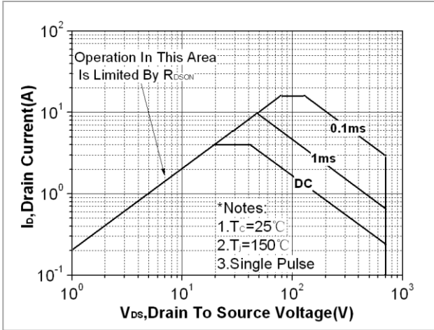
Fig. 7. Maximum safe operating area (TO-251&TO-251N)
