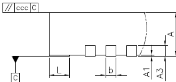
DETAIL : "B"
