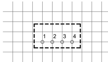
印刷板俯视图 Printed board vertical view 栅格间距 Latic spacing: 2.54mm(0.1inch)
