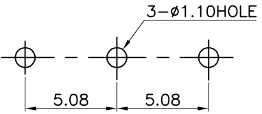
Recommended PCB Layout(Pattern Side) Top View tolerance: ±0.05mm
