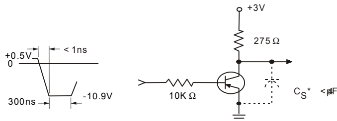
Delay and Rise Time Equivalent Test Circuit
