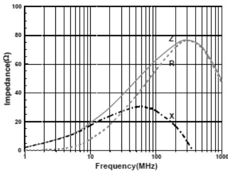
CMBH2012S600RSP
