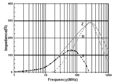
CMBH2012S301MSP
