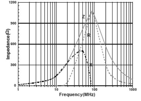
CMBH2012S102JSP
