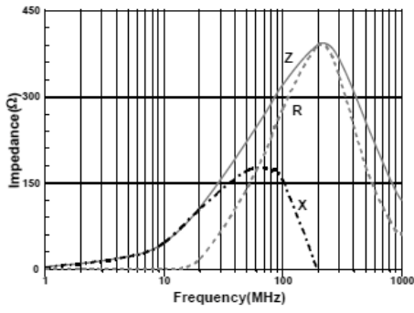
CMBH2012S331PSP
