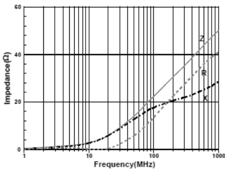
CMBH2012S600RSP
