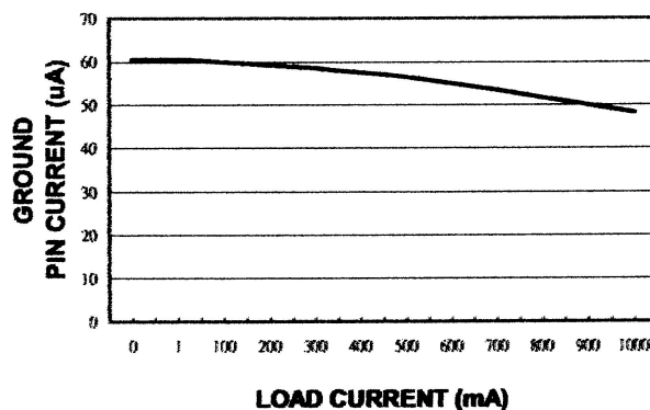
GROUND PIN CURRENT vs. LOAD CURRENT
