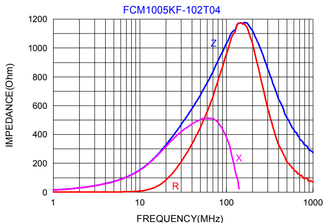
■ Impedance-Frequency Characteristics
