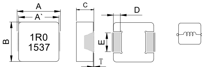
non-leadframe
