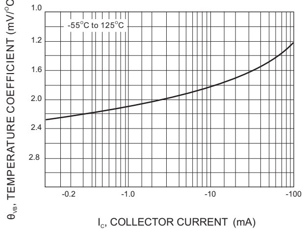
Fig. 10-BASE-EMITTER TEMPERATURE COEFFICIENT
