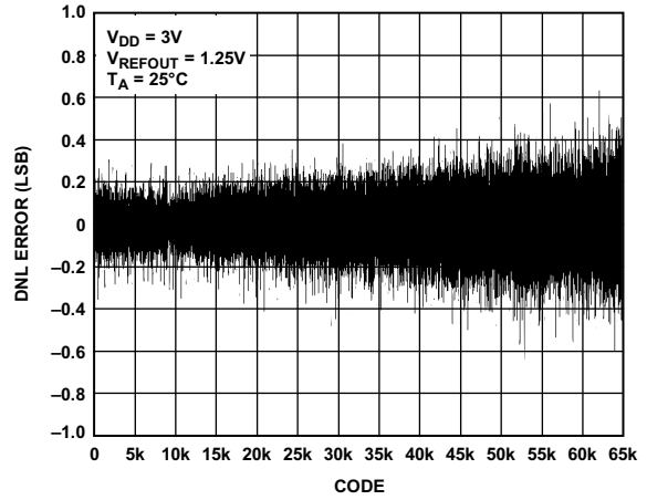
图19. DNL—AD5663R-3
