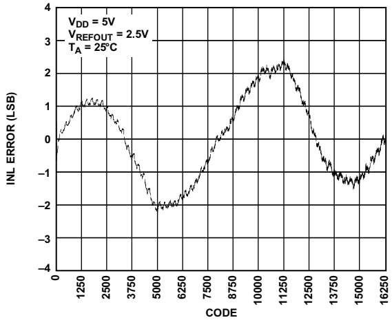
图11. INL—AD5643R-5
