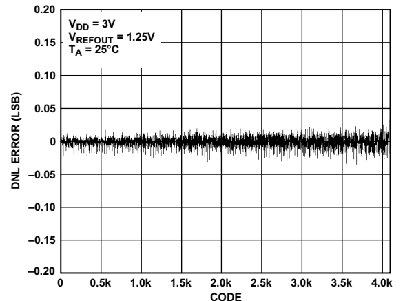
图21. DNL—AD5623R-3
