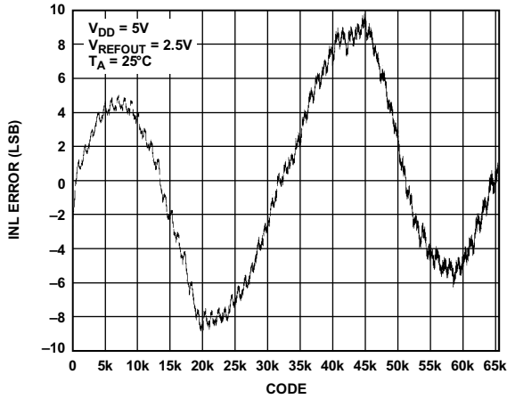
图10. INL—AD5663R-5
