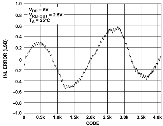
图12. INL—AD5623R-5
