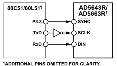
图58. AD5623R/AD5643R/AD5663R与80C51/80L51接口
