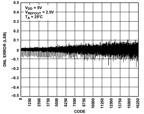
图14. DNL—AD5643R-5
