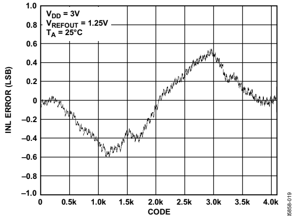
图18. INL—AD5623R-3
