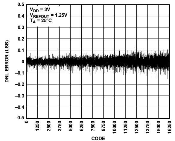
图20. DNL—AD5643R-3
