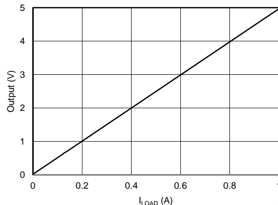
Figure 33. Low-Side, Current-Sense Transfer Function
