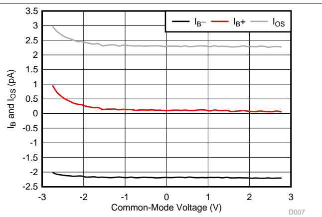
Figure 2. I_B and I_{OS} vs Common-Mode Voltage
