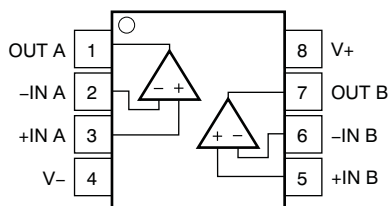
LMV358A D, DGK, PW Packages 8-Pin SOIC, VSSOP, TSSOP Top View
