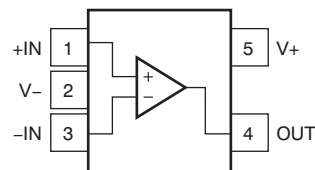
LMV321A DCK Package 5-Pin SC70 Top View
