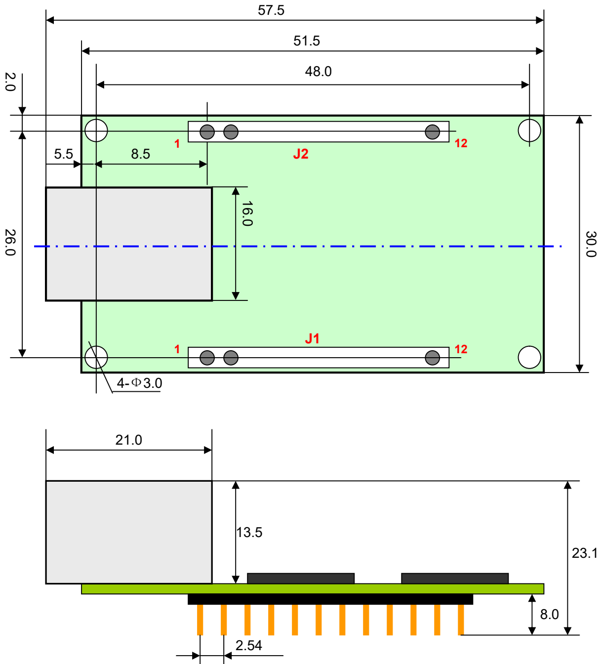
图2.1 HS-ENG091B尺寸图
