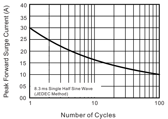
Fig.4 Maximum Non-Repetitive Peak Forward Surae Current
