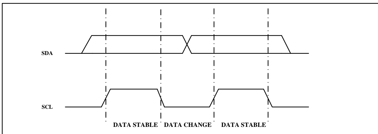
Figure 2. Data Validity
