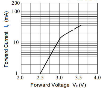
Fig.4-Forward Current vs. Forward Voltage T_a=25^{\circ}\text{C}
