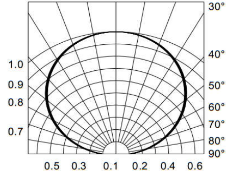
Fig.6-Radiation Diagram T_a=25^{\circ}\text{C}
