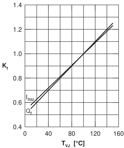
Fig. 4 Typ. dynamic parameters vs. junction temperature
