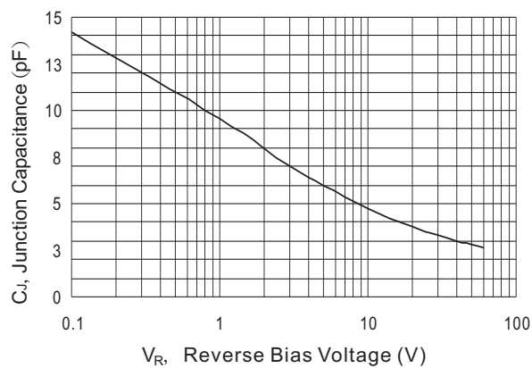
Fig.2-TYPICAL JUNCTION CAPACITANCE
