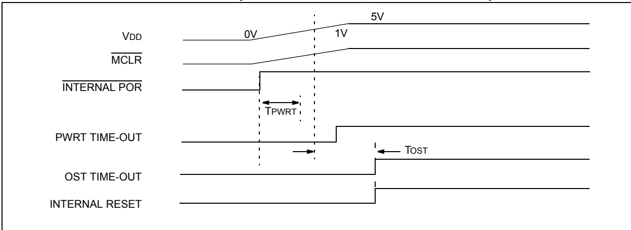
FIGURE 5-6: SLOW RISE TIME ( \overline{\text{MCLR}} TIED TO V_{\text{DD}} , V_{\text{DD}} RISE > TP_{\text{WRT}} )
