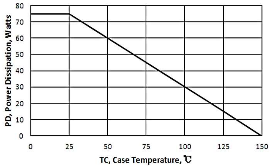
Figure 2 Maximum Power Dissipation vs Case Temperature
