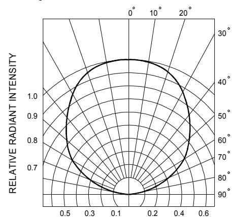
Fig.6 RADIATION DIAGRAM
