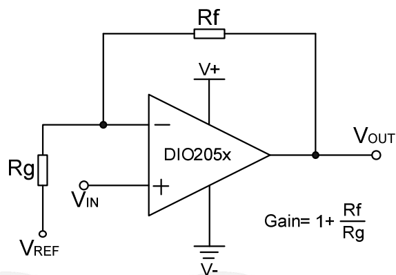
Non-Inverting Amplifier
