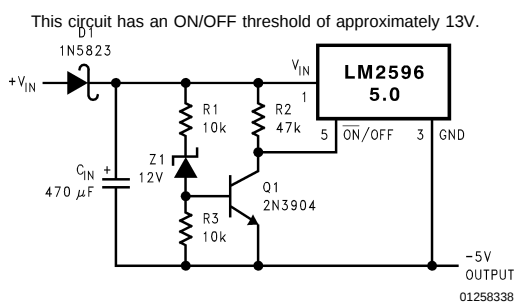
FIGURE 23. Undervoltage Lockout
