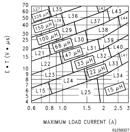
FIGURE 7. LM2596-ADJ
