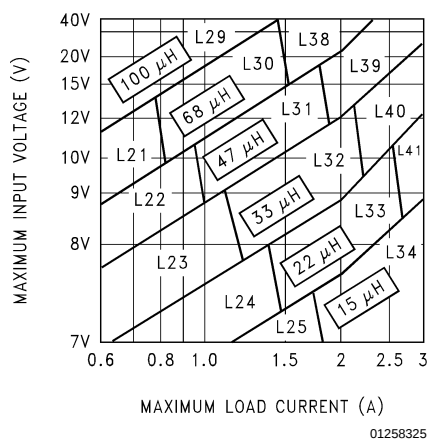
FIGURE 5. LM2596-5.0
