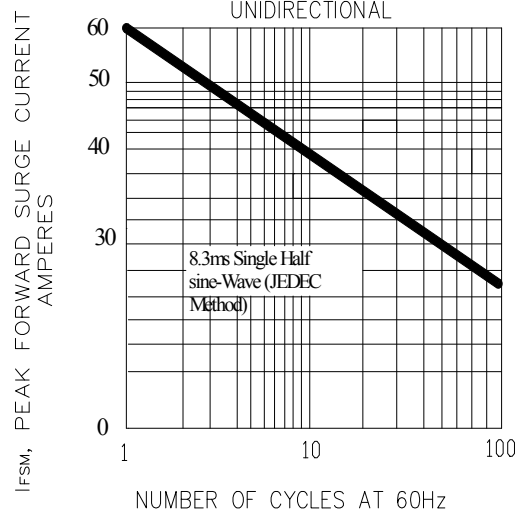
FIG.6- MAXIMUM NON-REPETITIVE FORWARD SURGE CURRENT UNIDIRECTIONAL
