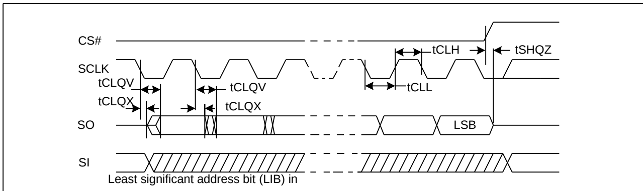
Figure22. Output Timing
