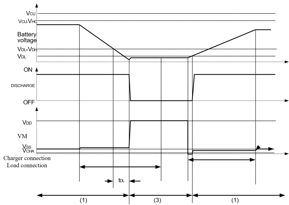
Figure5-3 Charger Detection
