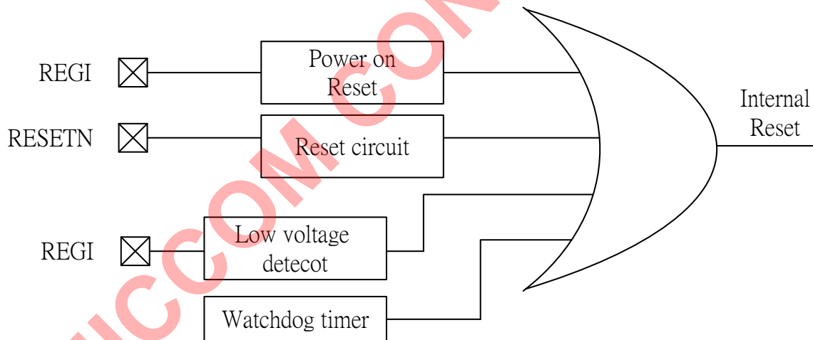
Figure 10.2 Reset source
