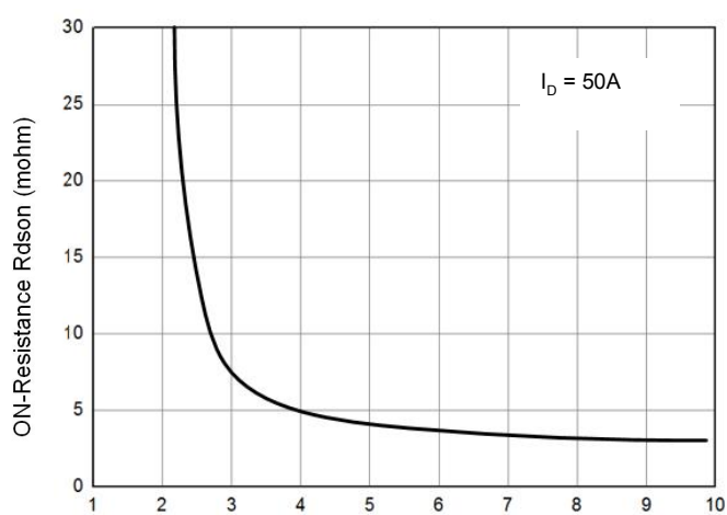
Figure 8. R_{DS(on)} vs Gate Voltage
