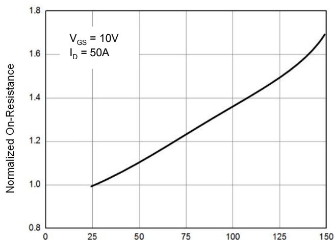
Figure 7. R_{DS(on)} -Junction Temperature( ^{\circ}\text{C} )
