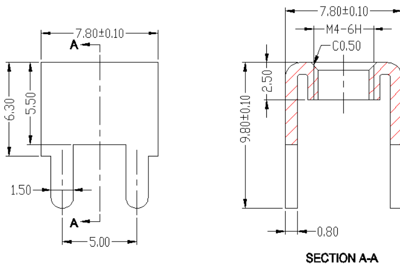
外形尺寸 (Shape Dimension)
