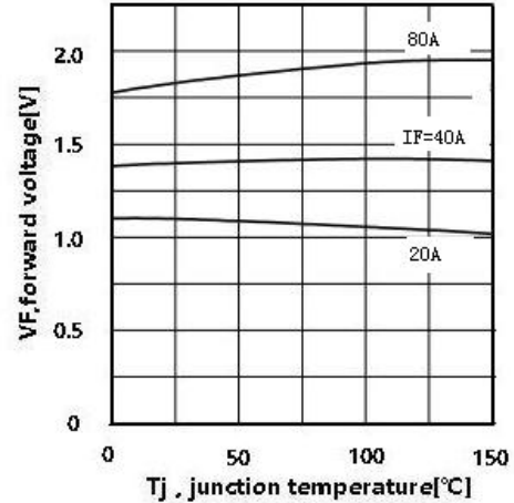
Figure 8 V_F vs. temperature
