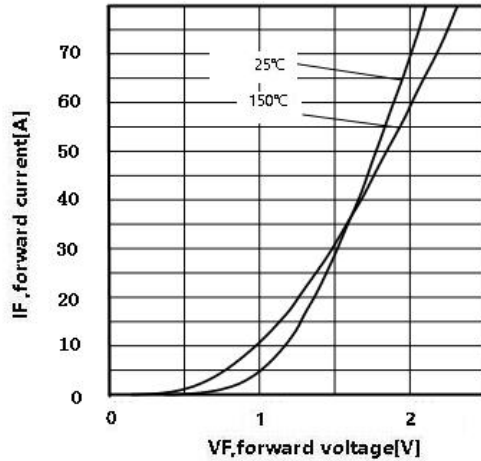
Figure 7. Forward Characteristics
