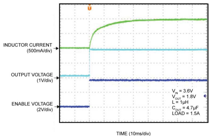
Start-Up Waveform
