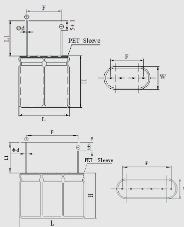
两端引出式产品外形示意图: Shape of wire lead supercapacitor:
