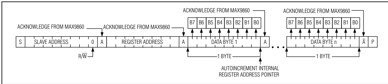
Figure 10. Writing N Bytes of Data to the MAX9860
