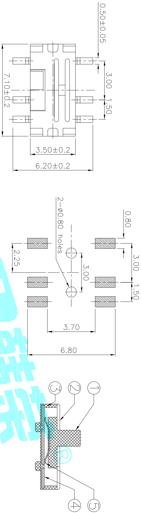
PCB Layout (Pattern side)
