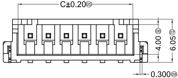
3P~16P Shape SCALE 1:1
