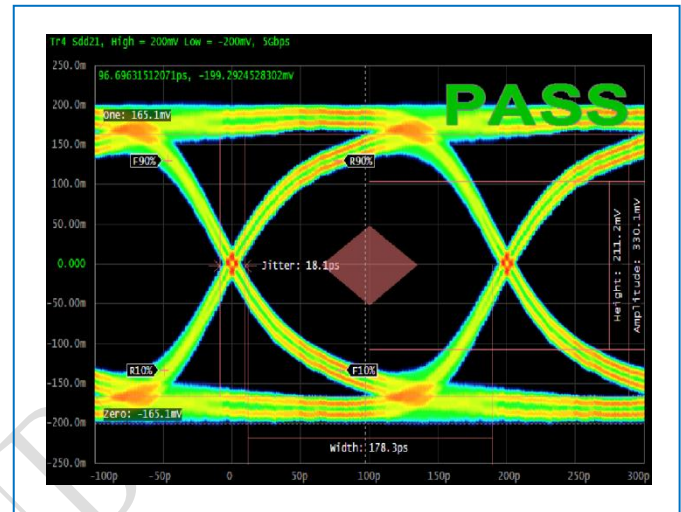
USB3.0 Mask at 5.0 Gbps
