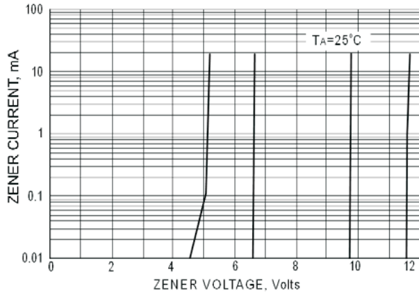
FIG. 5-ZENER BREAKDOWN CHARACTERISTICS
