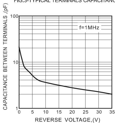
FIG.3-TYPICAL TERMINALS CAPACITANCE
