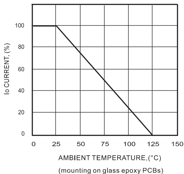
FIG.4- DERATING CURVE
