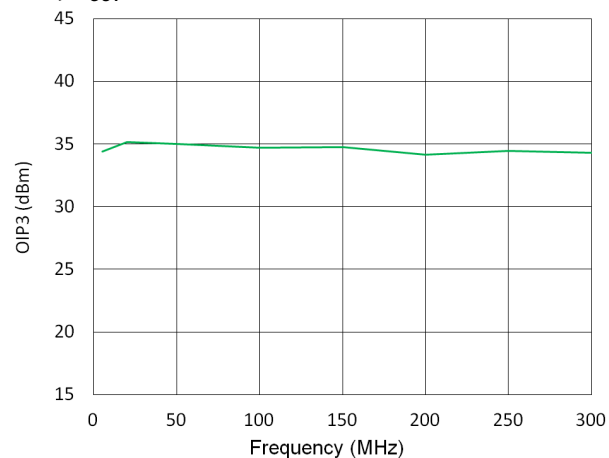
OIP3, P_{OUT} = 0\text{ dBm/ton}
