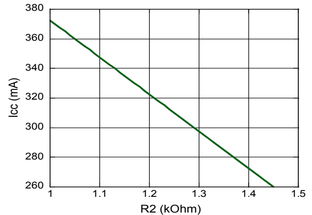
I_{CC} vs. Resistor R2 at V_{CC} = 5 V
