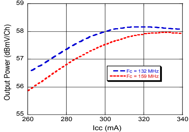
Output Power at 30 dB MER vs. I_{CC} 11
