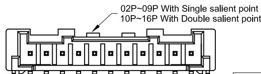
9P-16P SCALE 1:0.8
