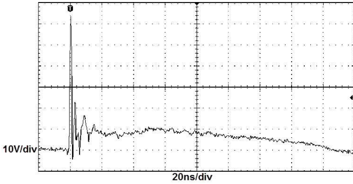
ESD clamping
