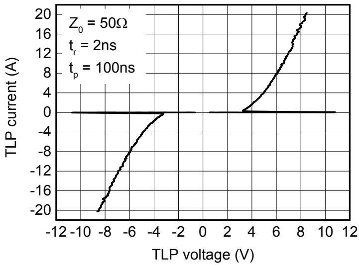
TLP Measurement
