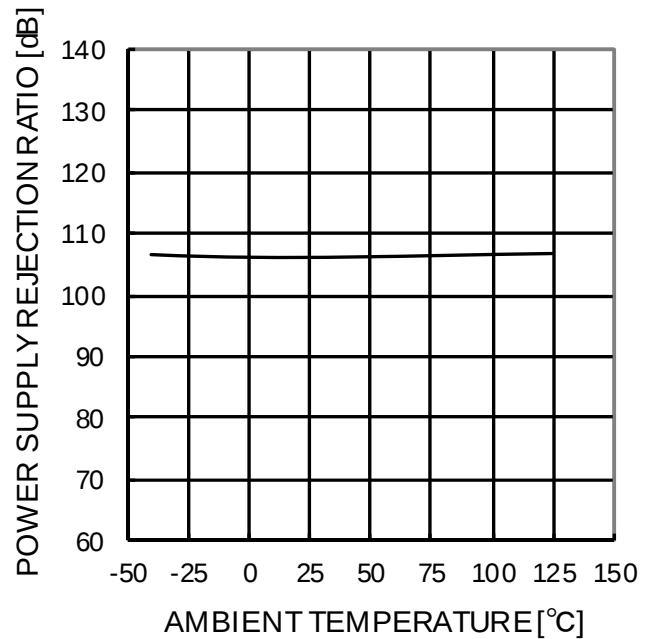
Figure 97. Power Supply Rejection Ratio - Ambient Temperature
