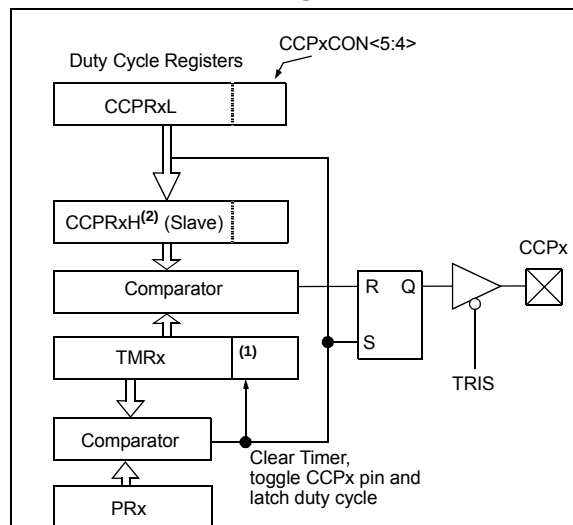
FIGURE 20-4: SIMPLIFIED PWM BLOCK DIAGRAM
