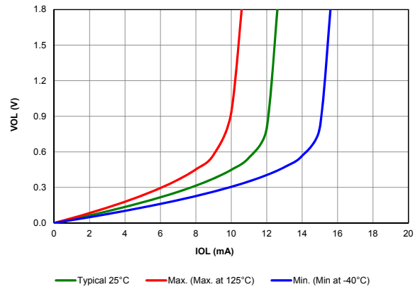
Figure 40-82. VOL vs. IOL OVER TEMPERATURE, V_{DD} = 1.8V
