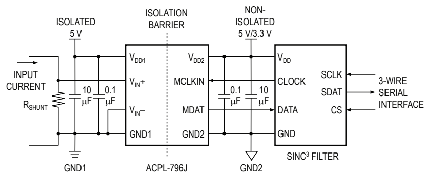
Figure 16. Typical application circuit with a Sinc 3 filter.
