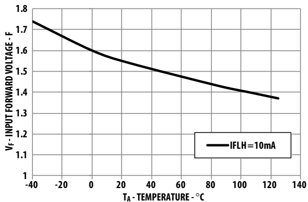
Figure 7. V_F vs. Temperature
