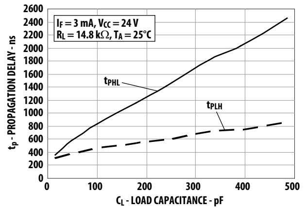
Figure 21 Typical Propagation Delay vs. Load Capacitance (ACPL-054L/W50L/K54L)
