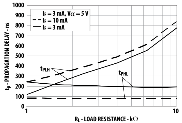
Figure 19 Typical Propagation Delay vs. Load Resistance
