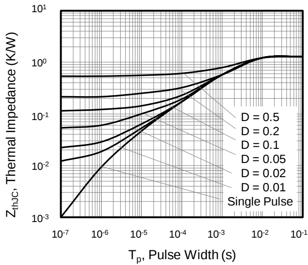
Figure 9. Transient Thermal Impedance TO-262, TO-251, TO-252
