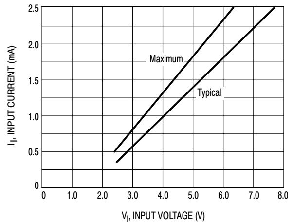
Figure 6. Input Characteristics
